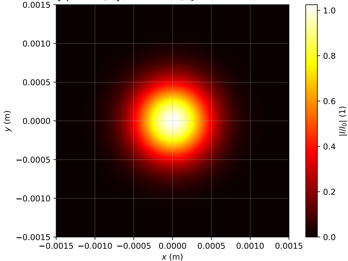
Intensity profile I(x, y, z = 0.239m)/I_0 , P_{in}=0.7P_{cr} , artificial time
